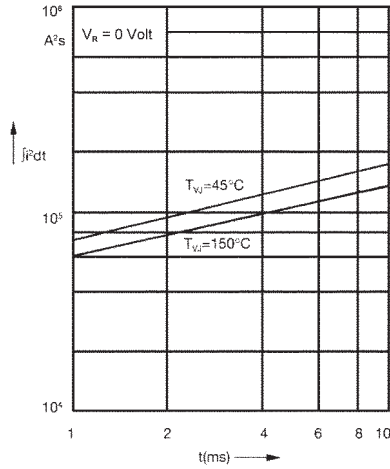
Fig. 2 \int i^2 dt versus time (1-10 ms)
