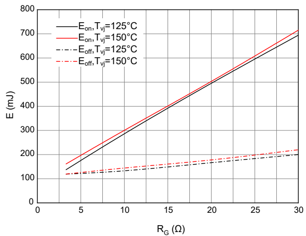
Figure 6. Switching losses of IGBT
