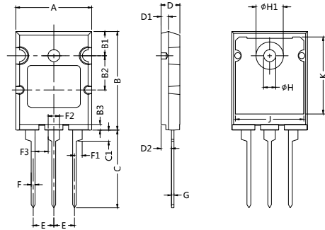
TO-264
