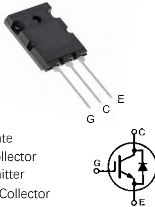
TO-264
