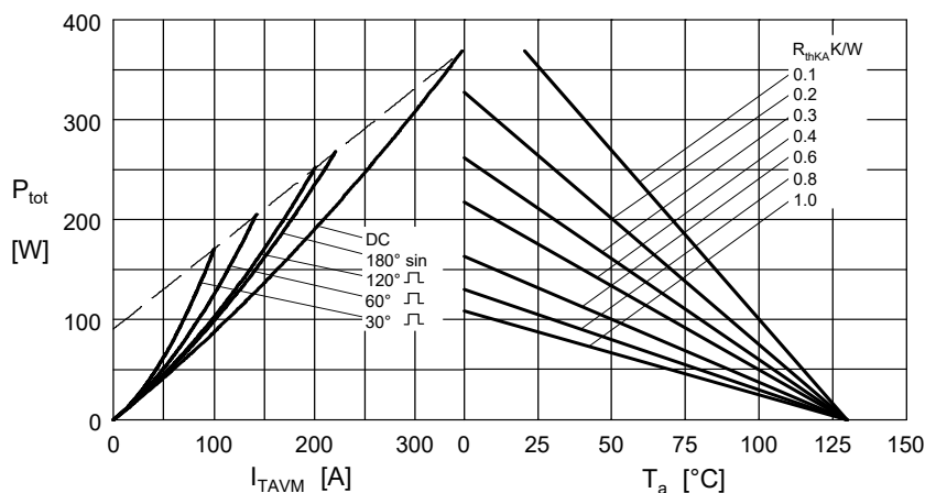
Fig. 4 Power dissipation vs. on-state current & ambient temperature (per thyristor or diode)
