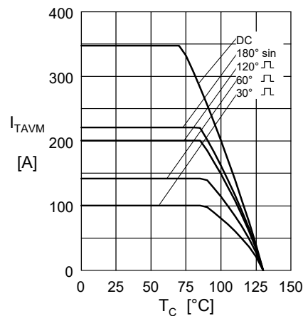
Fig. 3 Max. forward current at case temperature
