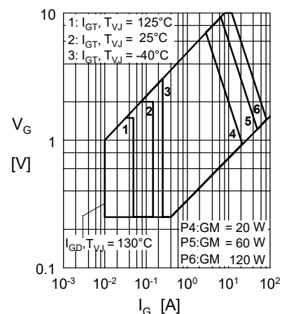
Fig. 5 Gate trigger characteristics
