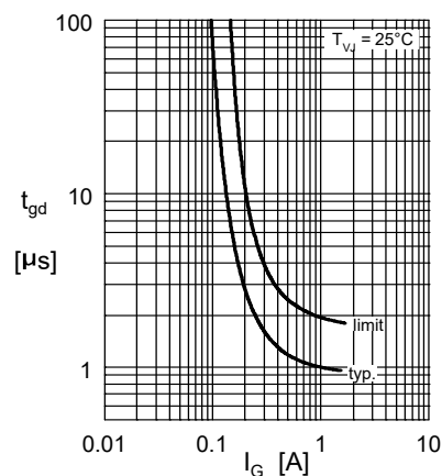
Fig. 7 Gate trigger delay time
