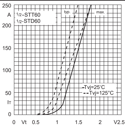
Fig.7 On-state characteristics
