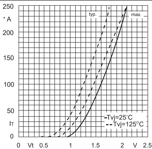
Fig.7 On-state characteristics
