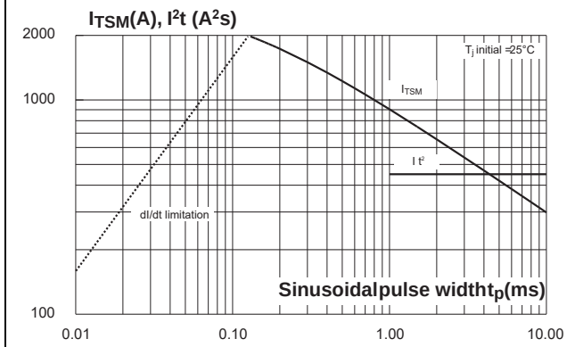
Figure 8. Non-repetitive surge peak on-state current, and corresponding values of I^2t
