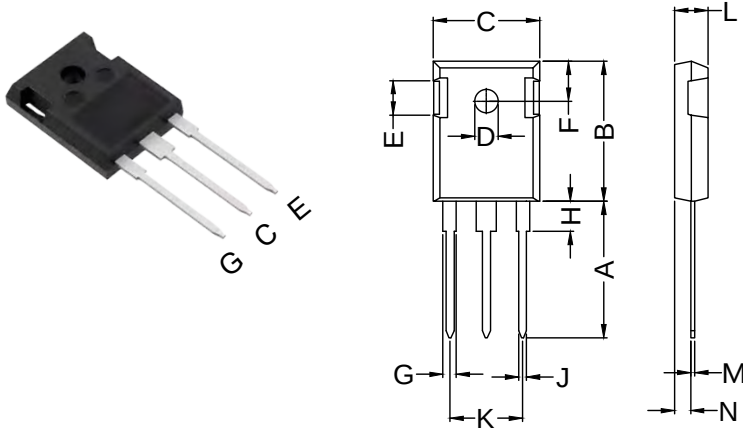
Dimensions TO-247AD
