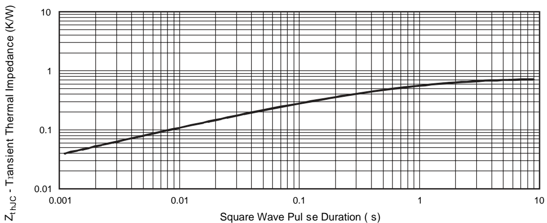
Fig. 4 - Thermal Impedance Z_{thJC} Characteristic
